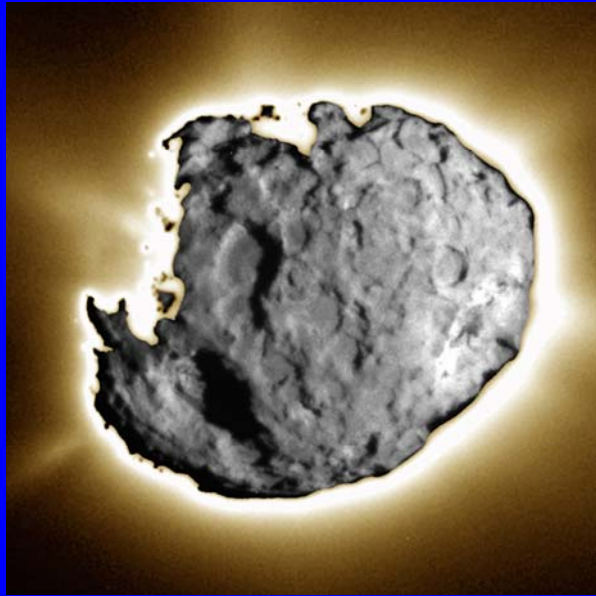
Composite image of comet Wild 2 taken by Stardust
