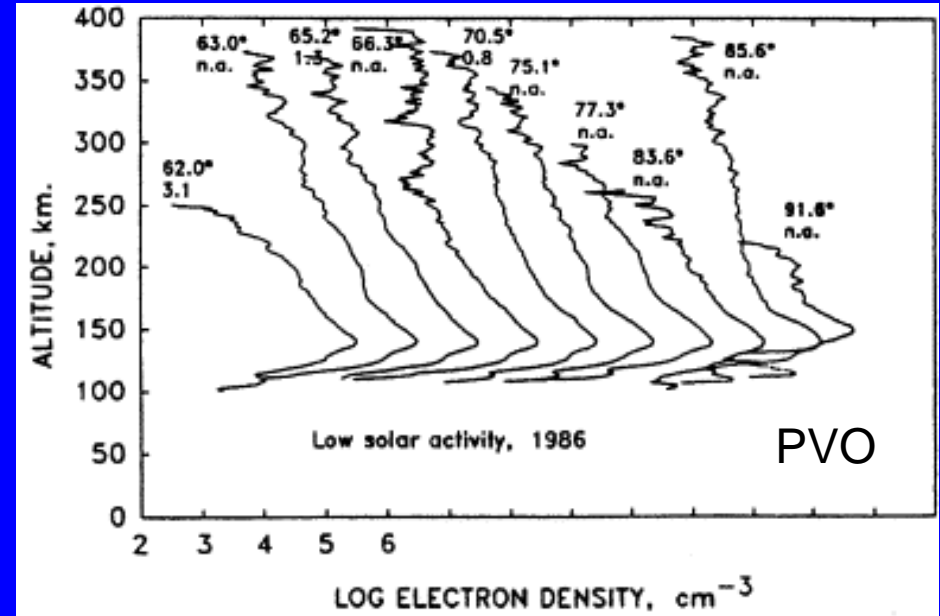
Figure 4 of Kliore (1992)
