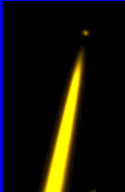
Artificial guide star produced by 589 nm laser
